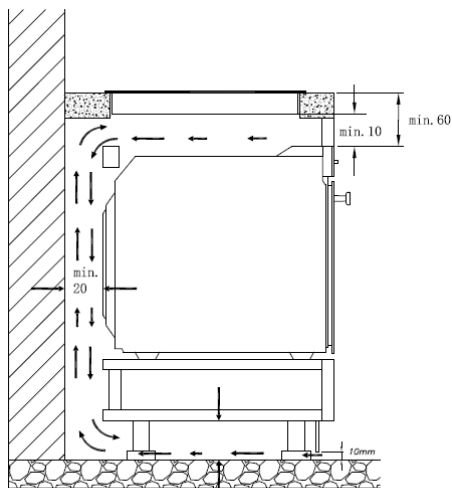
Oven base
