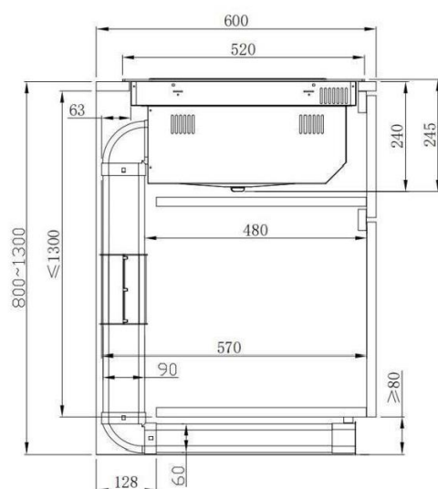
Filtration Version
