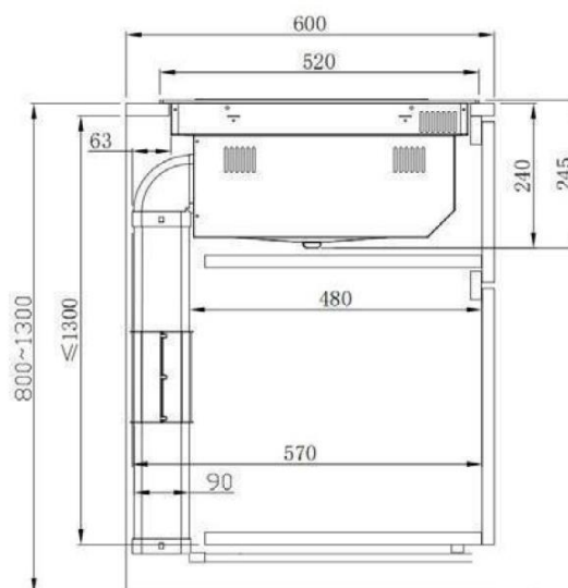
Exhausting Version
