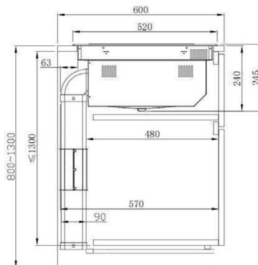
Utsugningsversion
