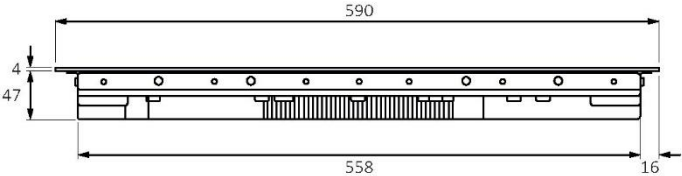
Vista frontal
