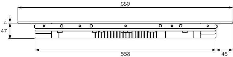
Vista frontal
